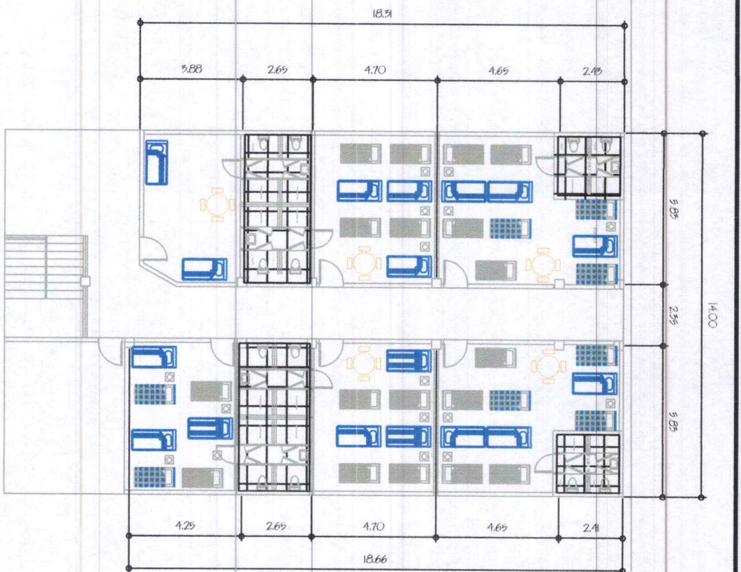
TILE PLAN-SECOND FLOOR
