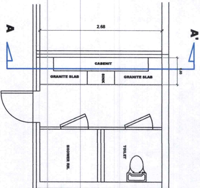
COMFORT ROOM "A" PLAN SCALE 1: 80 MTS.
